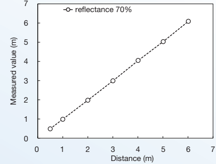
Distance accuracy
