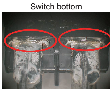
Switch bottom Flux adheres to the terminal base
