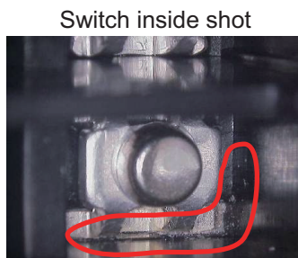
Switch inside shot Flux enters through the gap between the case and the terminal
