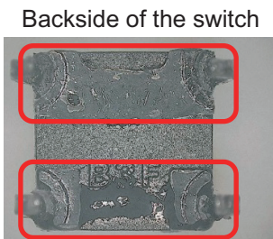
The resin is melted
