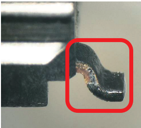
The terminal is discolored to black due to sulfurization
