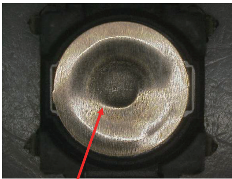
NG switch contact dome
