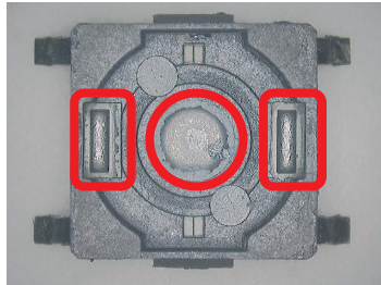
Contact parts are discolored to black due to sulfurization
