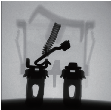
OK switch X-ray
