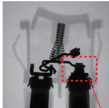
NG switch X-ray
