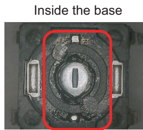
The resin is melted
